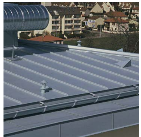
Air inlets and outlets are generally linear (at least 10mm wide) but can be individual (see photo). The ventilation must correspond to BS 5250: 2002.
